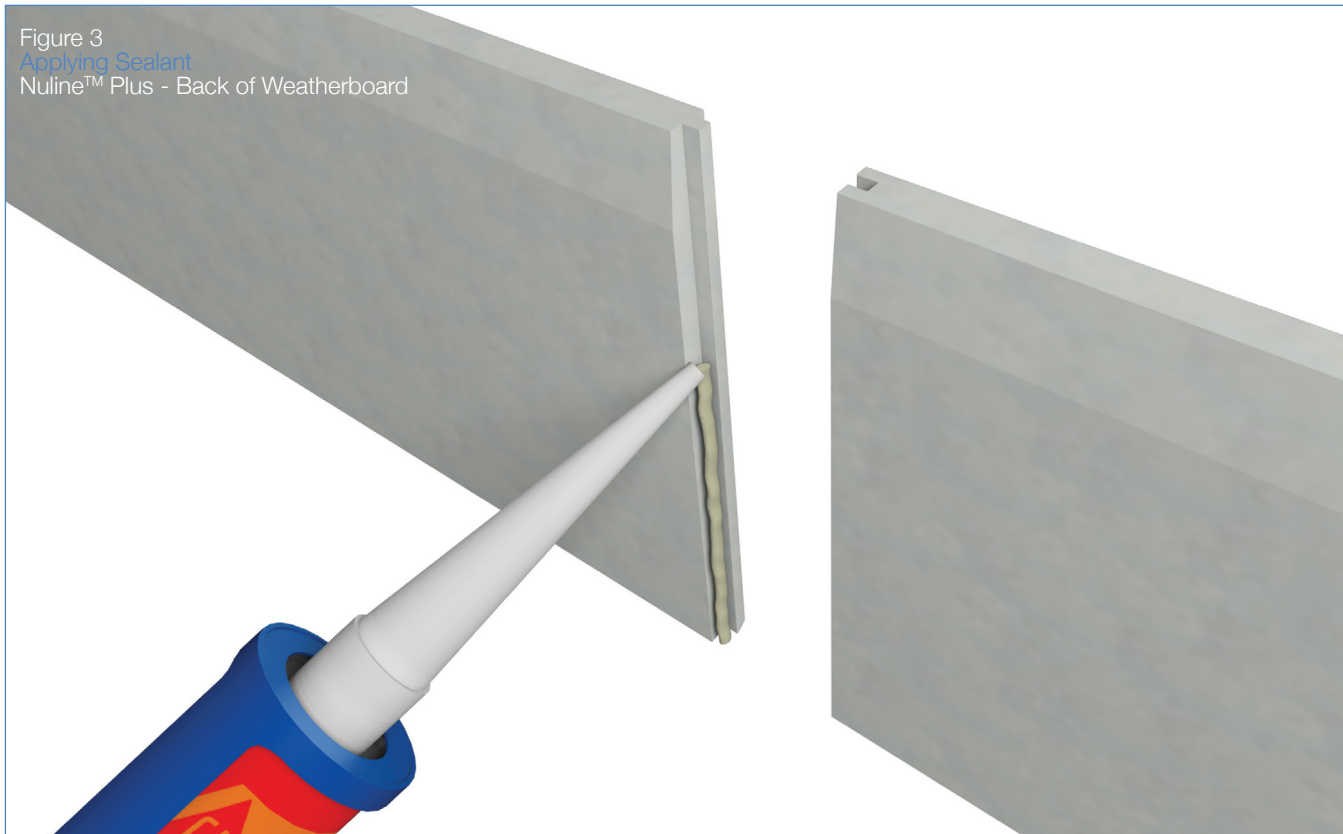
Figure 4 Joint Detail
