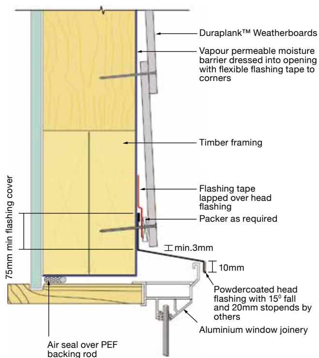
FIGURE 9 // WINDOW HEAD
