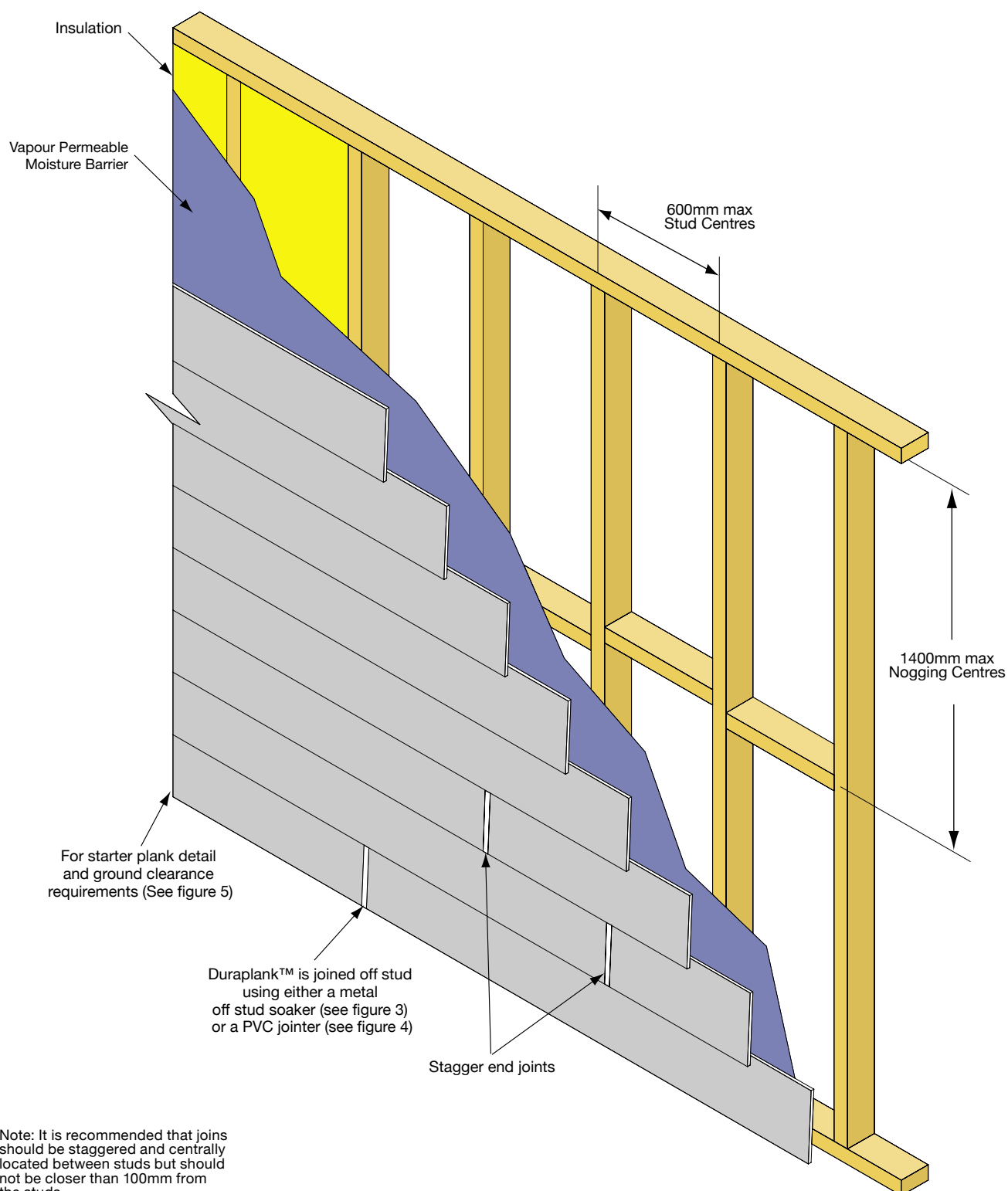
FIGURE 2 // DURAPLANK™ LAYOUT
