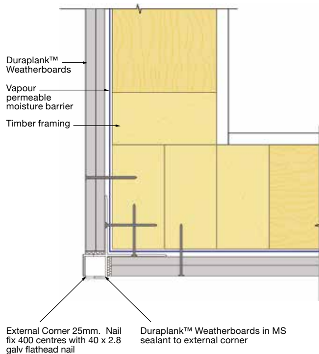
FIGURE 12 // EXTERNAL CORNER DETAIL WITH INNOVA PROFILE
