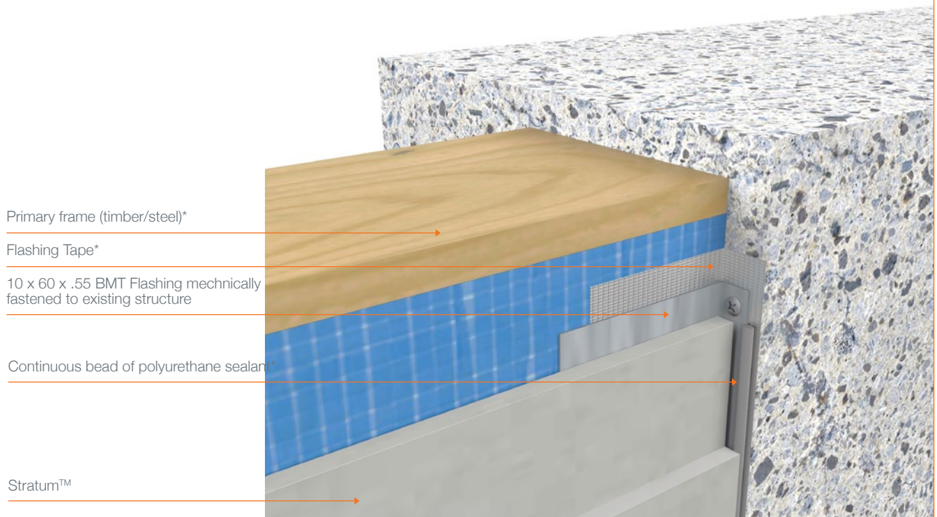
Figure 22 Stratum™ / Stratum™ Duo / Stratum™ Trio Wall Abutment
