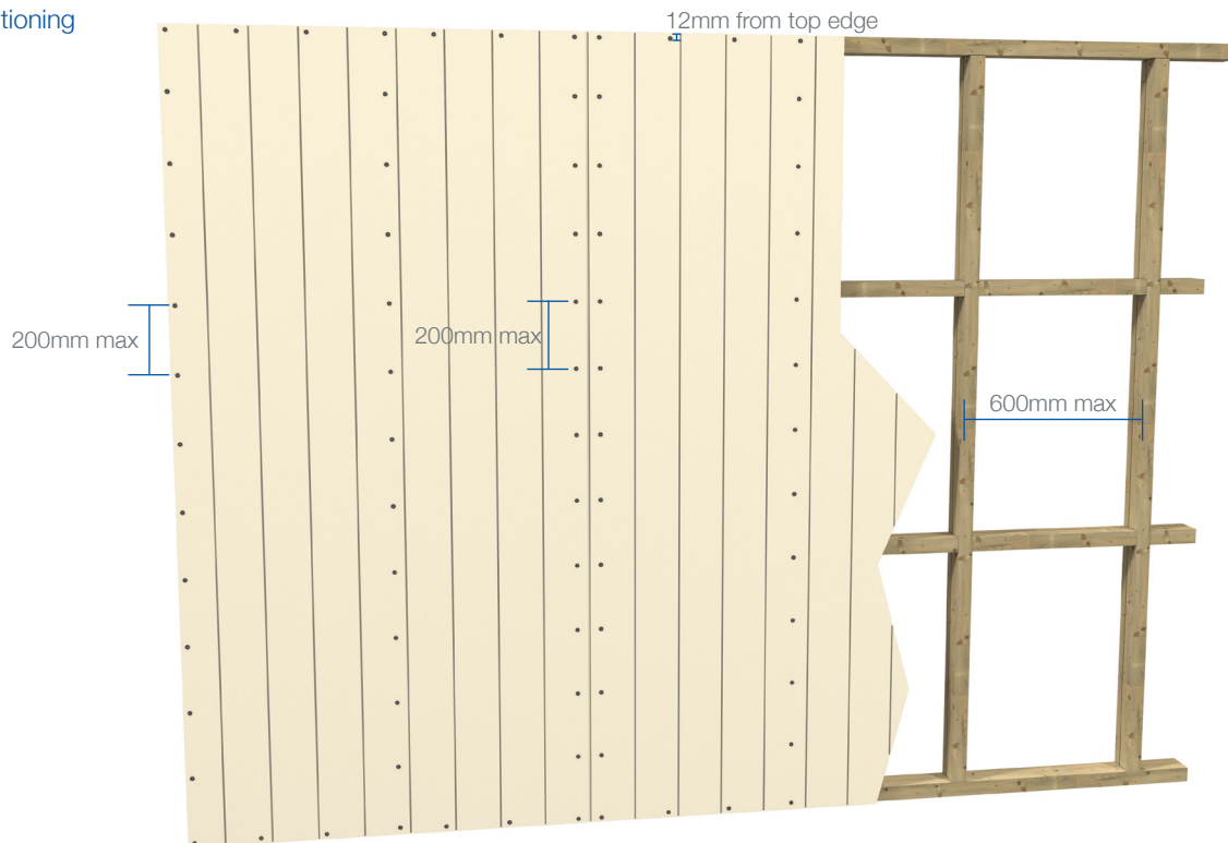
Figure 4 Fastener Positioning
