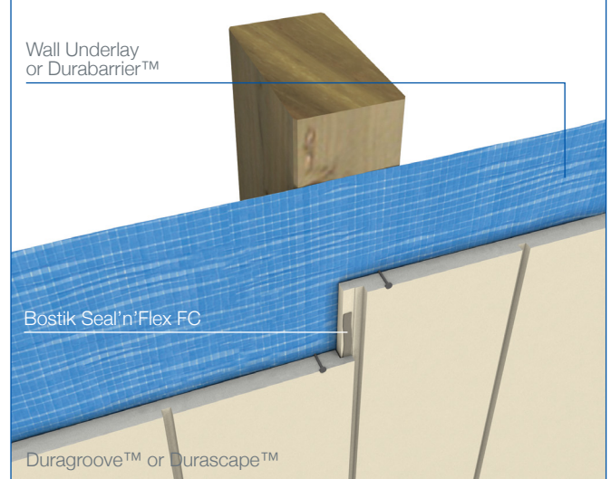
Figure 3 Fibre Cement Nail/Brad Fixing – Direct Fix
