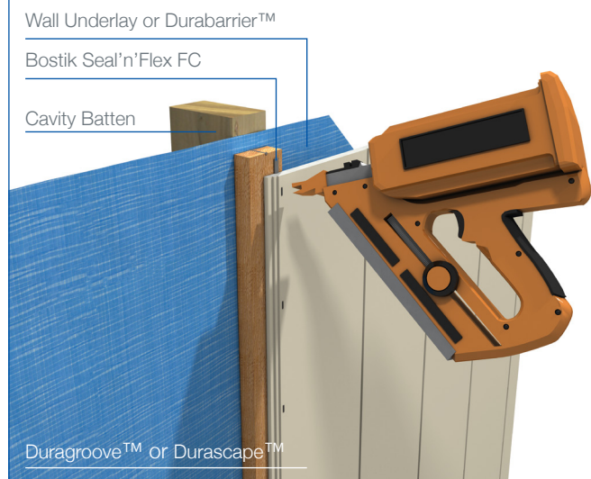
Figure 8 Fix Next Sheet
