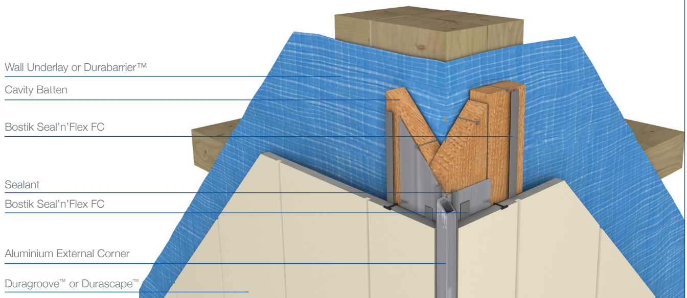
Figure 11 External Corner - Aluminium Profile
