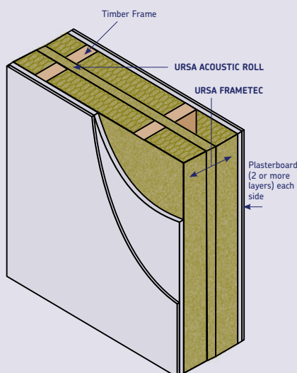
Figure 3 Timber Frame Separating Wall
