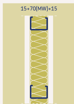
Gypsum board partition GB 100/600(70) P
