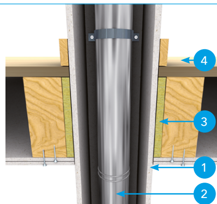
Principedetail.
