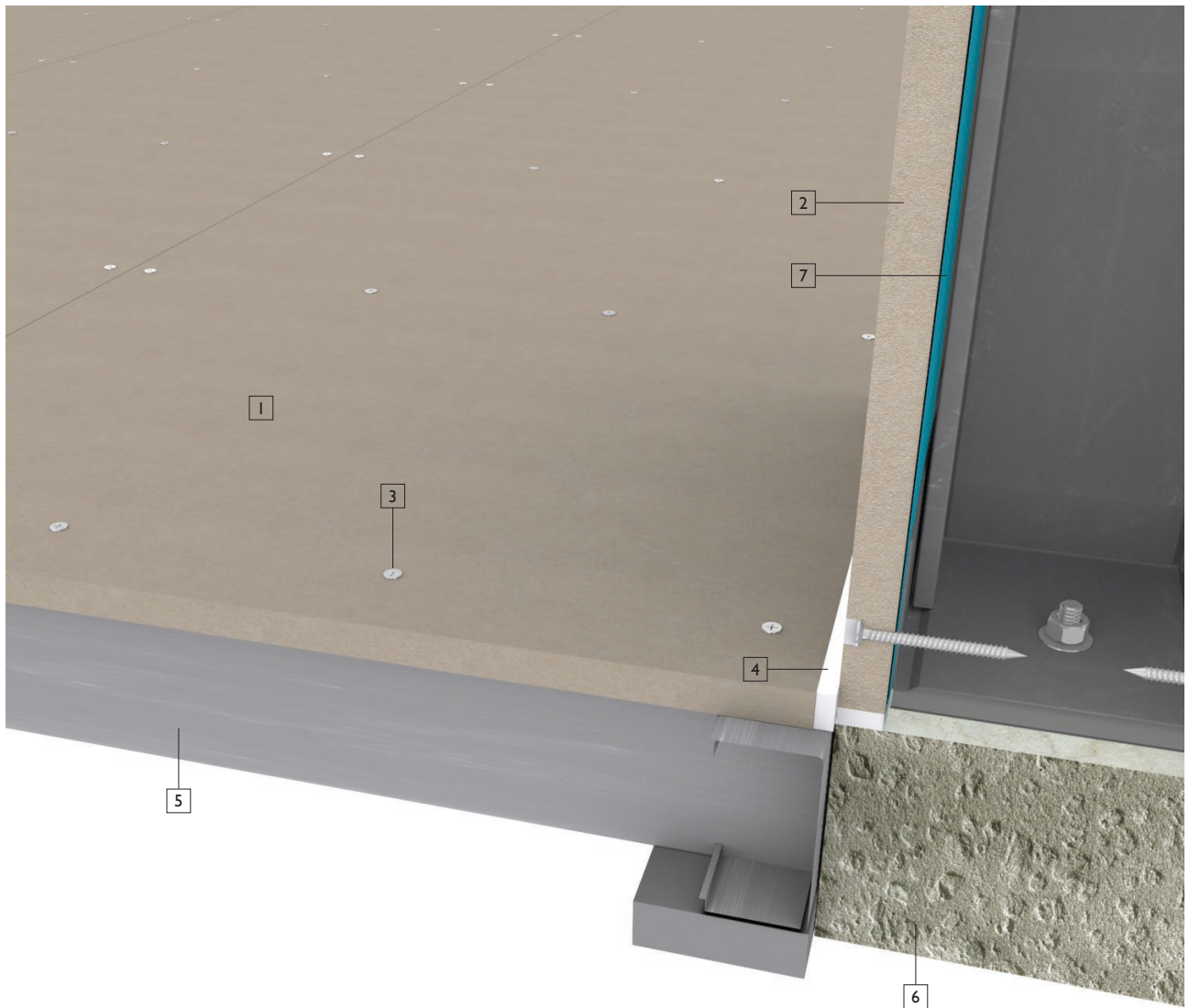
Figure 10 Wall and floor joint
