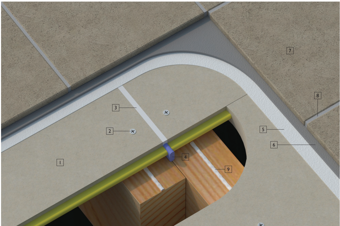
Figure 5 Control joints - Non wet area tiling
