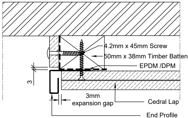
Plan on Profile 1:2 End Profile
