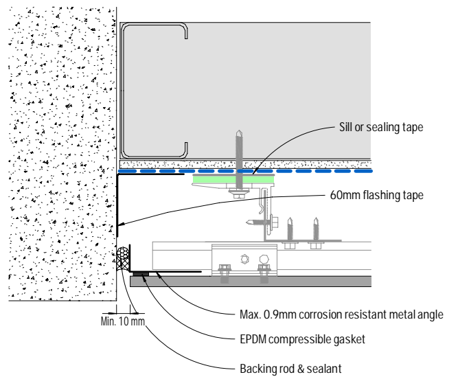
Figure 28: Abutment
