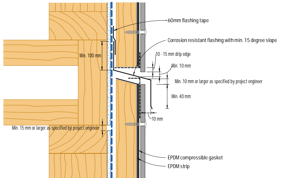
Figure 9: Horizontal control joint
