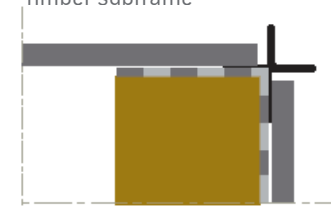
Figure 6: External Corner with trim Timber subframe
