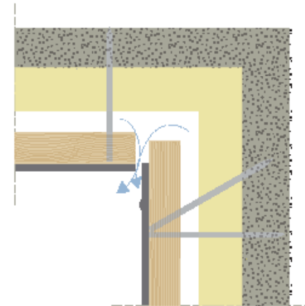
Figure 20: Soffit Detail
