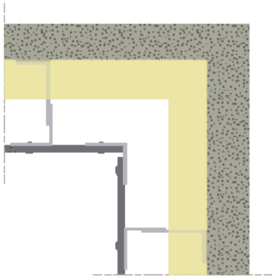
Figure 7: Robust Internal Corner Detail Metal
