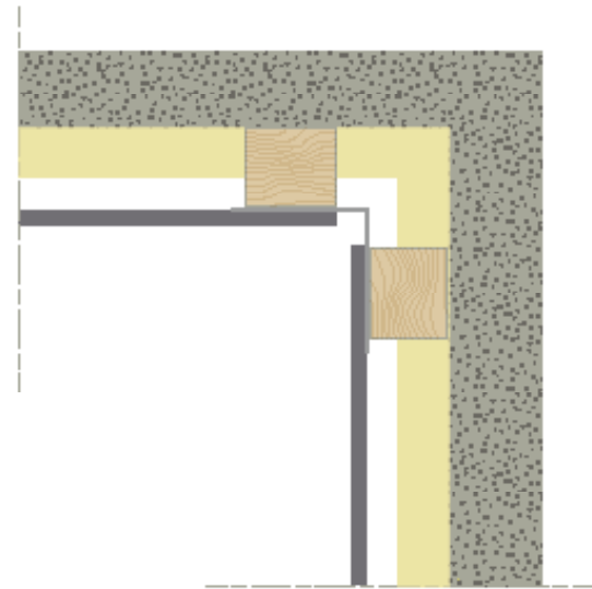
Figure 9: Alternative Internal corner trim Timber
