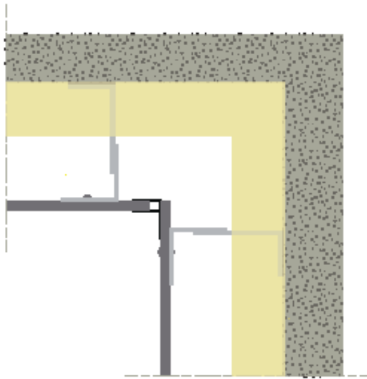
Figure 8: Internal corner trim Could be metal or plastic
