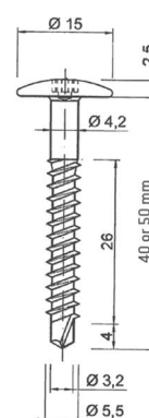
UNI Screw with drilling point tip
