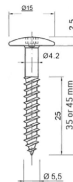
UNI Screw with standard tip
