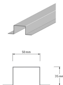
Typical intermediate top hat profile
