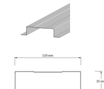
Typical joint top hat profile located at panel vertical joints
